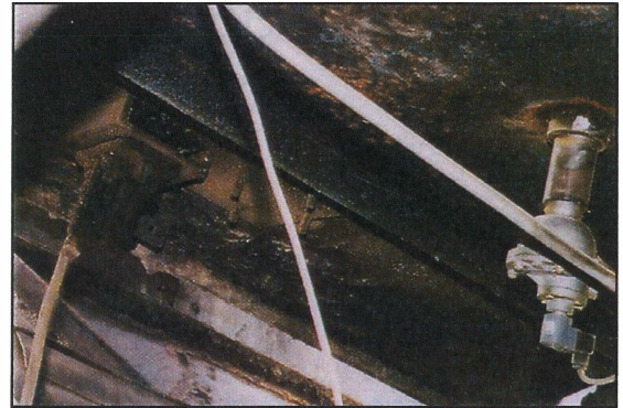
Past attempts to move fly ash with other equipment, such as the pneumatic vibrator shown on the left, proved ineffective. AirSweep unit is on the right.
